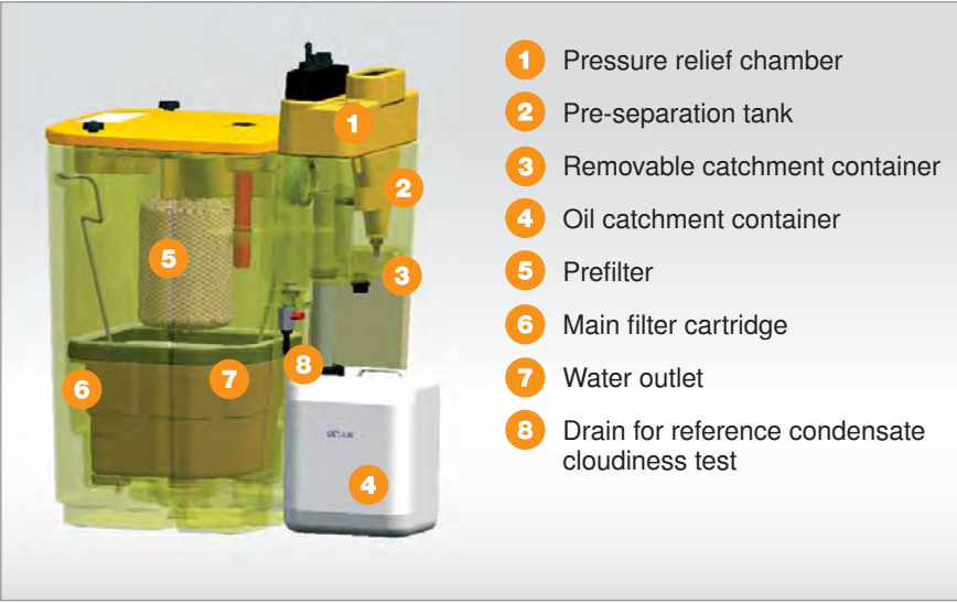
Fig. 2: Condensate separation system for compressed air technology using the gravity principle (functional diagram)
