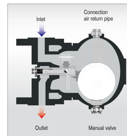
Fig. 4: Float drain for compressed air condensate
