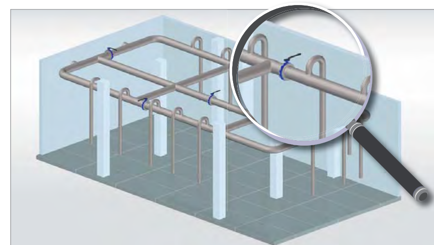
Fig. 3: Compressed air distribution network with pipeline grid
