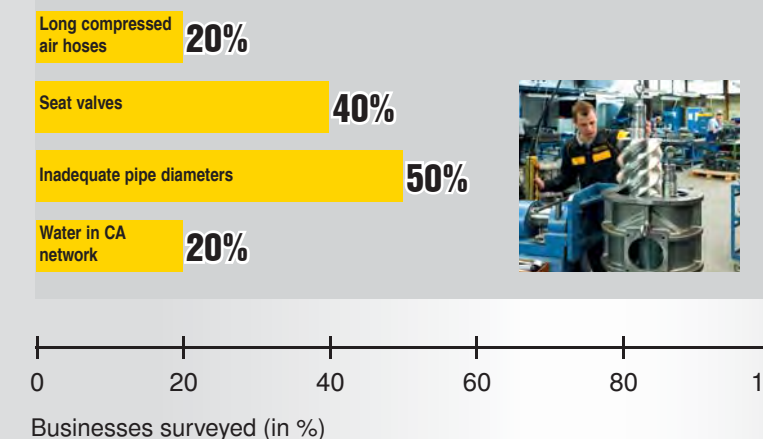
Fig. 3: For original findings, please refer to the results analysis of the compressed air audits performed by KAESER KOMPRESOREN within the scope of the 'Drucklufteffizient' campaign. Thesis: Anja Seitz, Coburg University, Specialism: Mechanical Engineering (2003)
