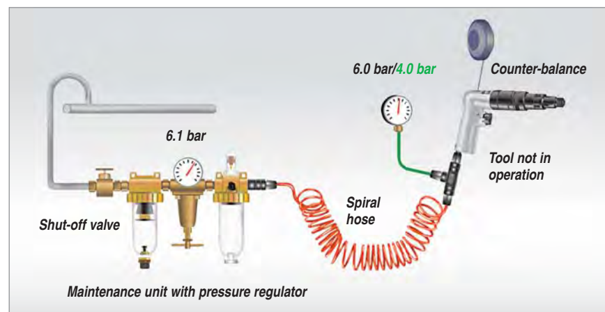
Caption: Tool connection with spiral hose – 6.0 bar pressure with zero compressed air consumption. 4.0 bar when tool in operation = 2 bar pressure drop when tool in operation: only 54 % of full performance capacity!
