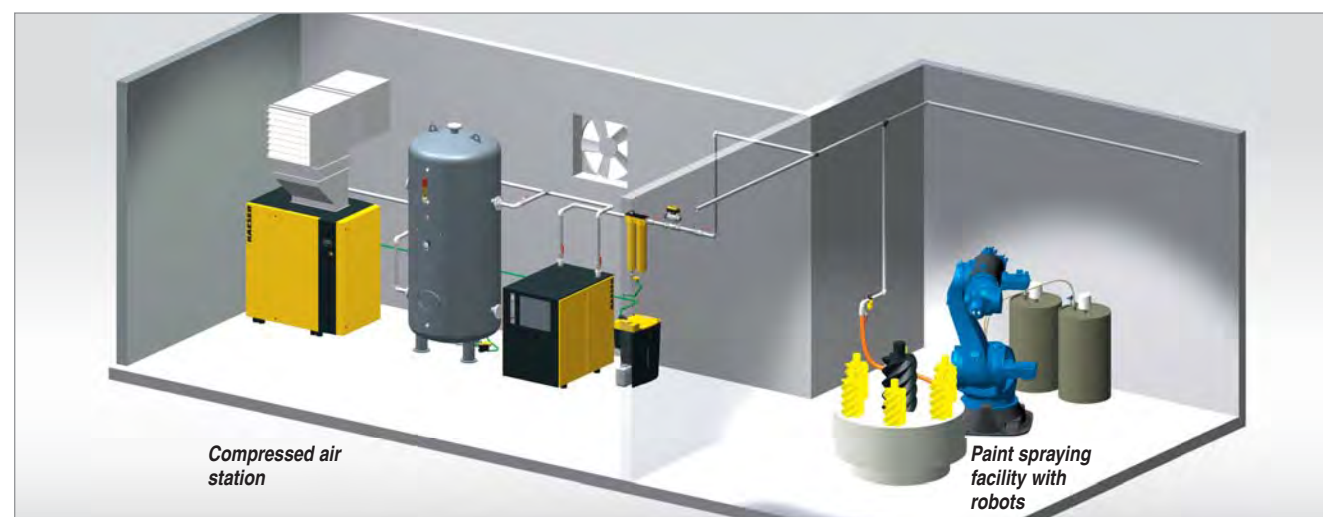
Fig. 5: Insightful: compressed air system inspection
