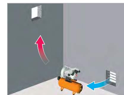
Fig. 1: Natural ventilation for compressors up to 5.5 kW
